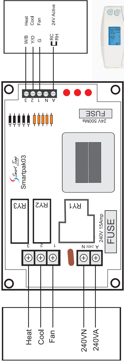
Typical One Stage Heat Cool A/C Unit
